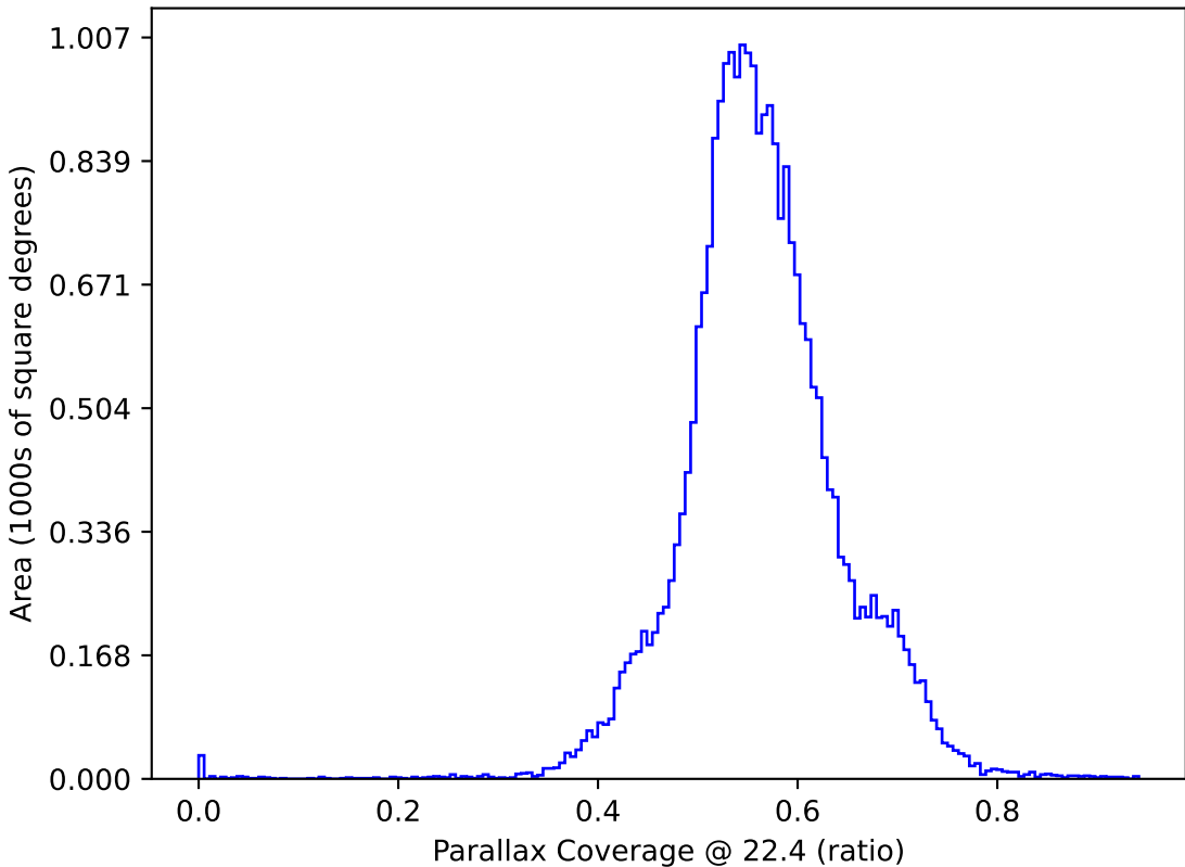
too_combined_s1.0_v3.4_10yrs : Parallax Coverage @ 22.4
