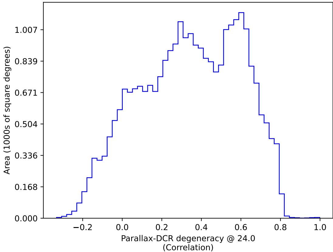
too_combined_s1.0_v3.4_10yrs : Parallax-DCR degeneracy @ 24.0
