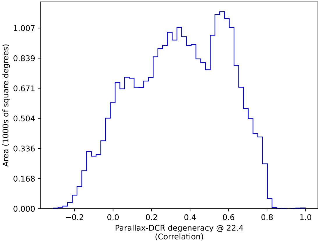
too_combined_s1.0_v3.4_10yrs : Parallax-DCR degeneracy @ 22.4
