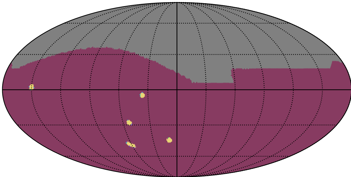
too_combined_s1.0_v3.4_10yrs : NumberOfQuickRevisits
