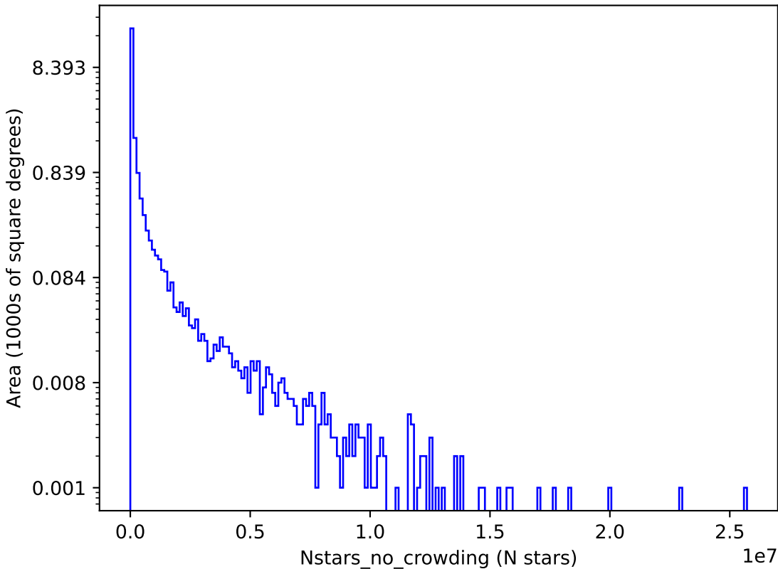
too_combined_s1.0_v3.4_10yrs y: Nstars_no_crowding
