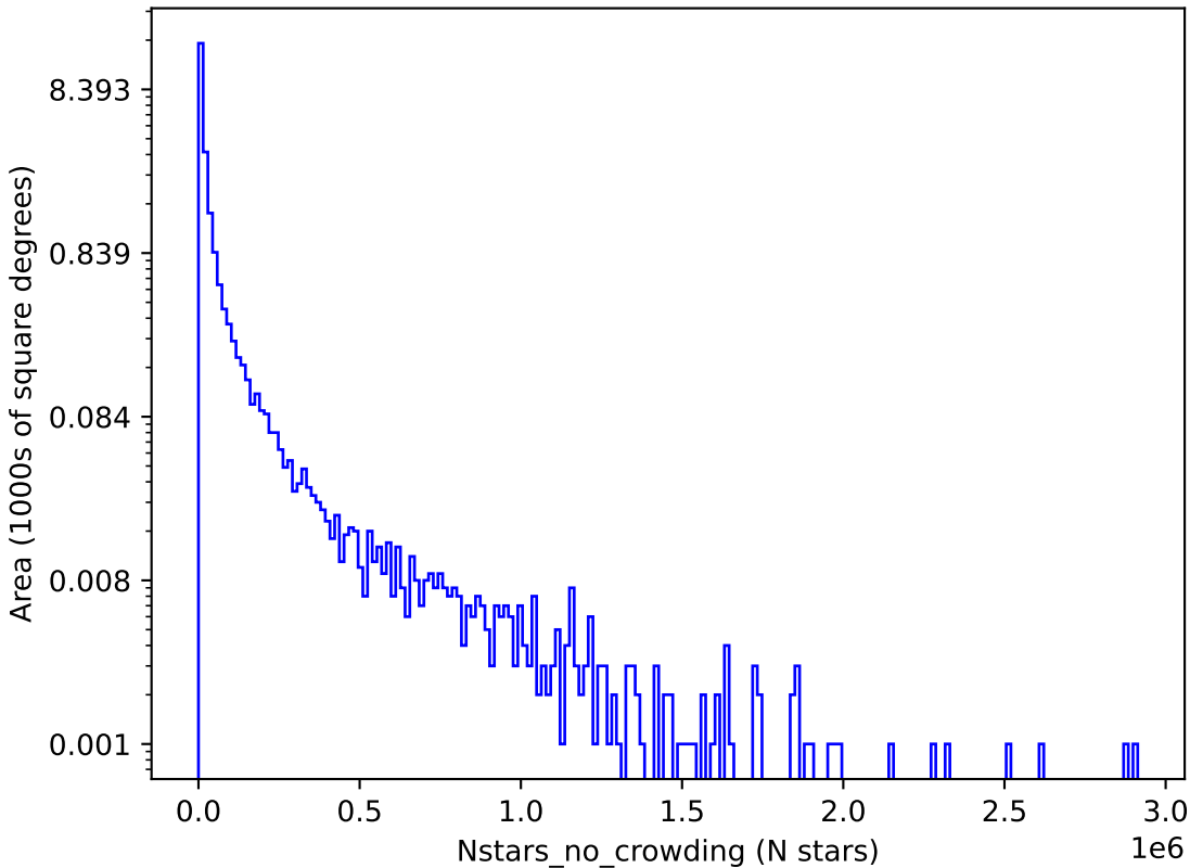
too_combined_s1.0_v3.4_10yrs u: Nstars_no_crowding
