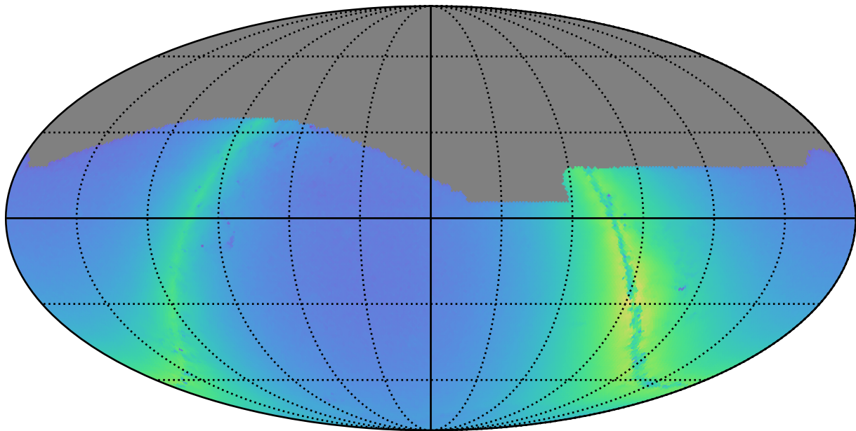
too_combined_s1.0_v3.4_10yrs r: Nstars_no_crowding
