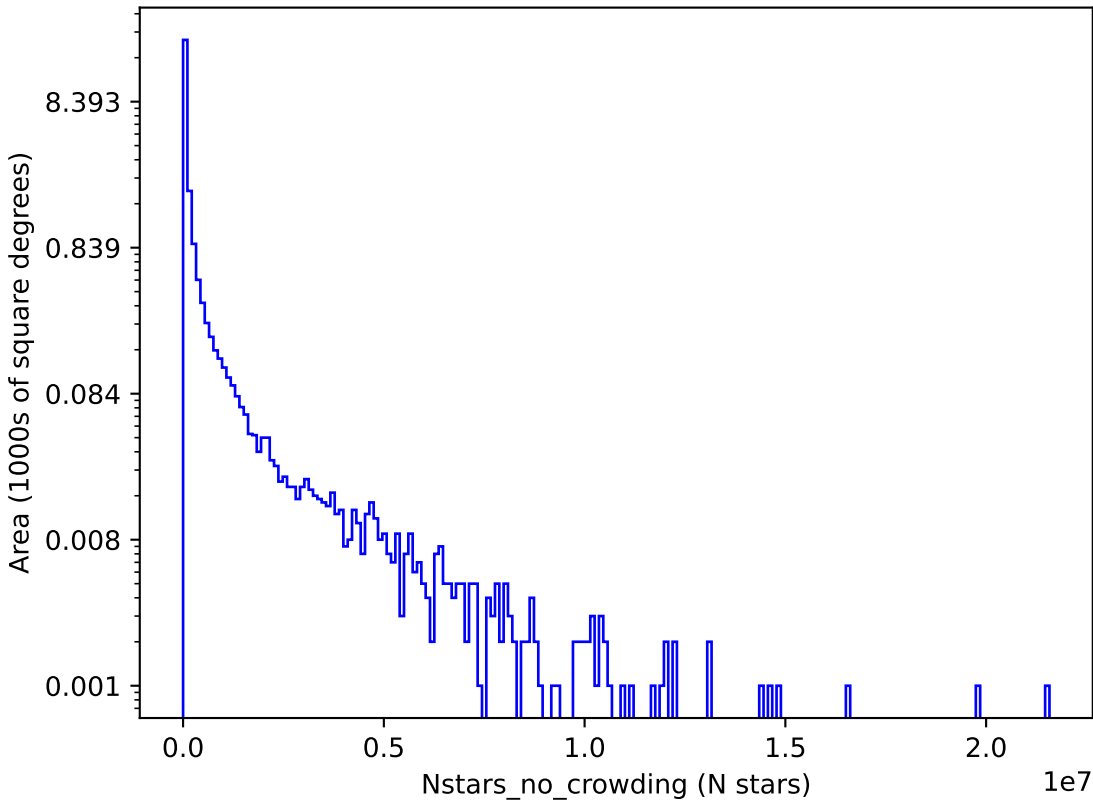
too_combined_s1.0_v3.4_10yrs r: Nstars_no_crowding
