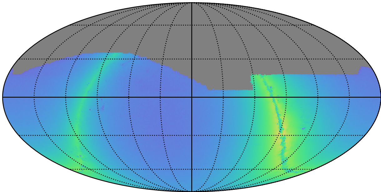
too_combined_s1.0_v3.4_10yrs i: Nstars_no_crowding
