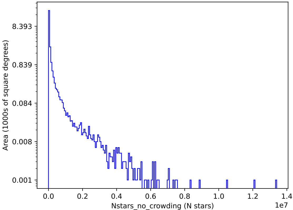
too_combined_s1.0_v3.4_10yrs g: Nstars_no_crowding
