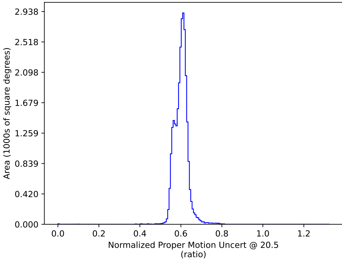
too_combined_s1.0_v3.4_10yrs : Normalized Proper Motion Uncert @ 20.5
