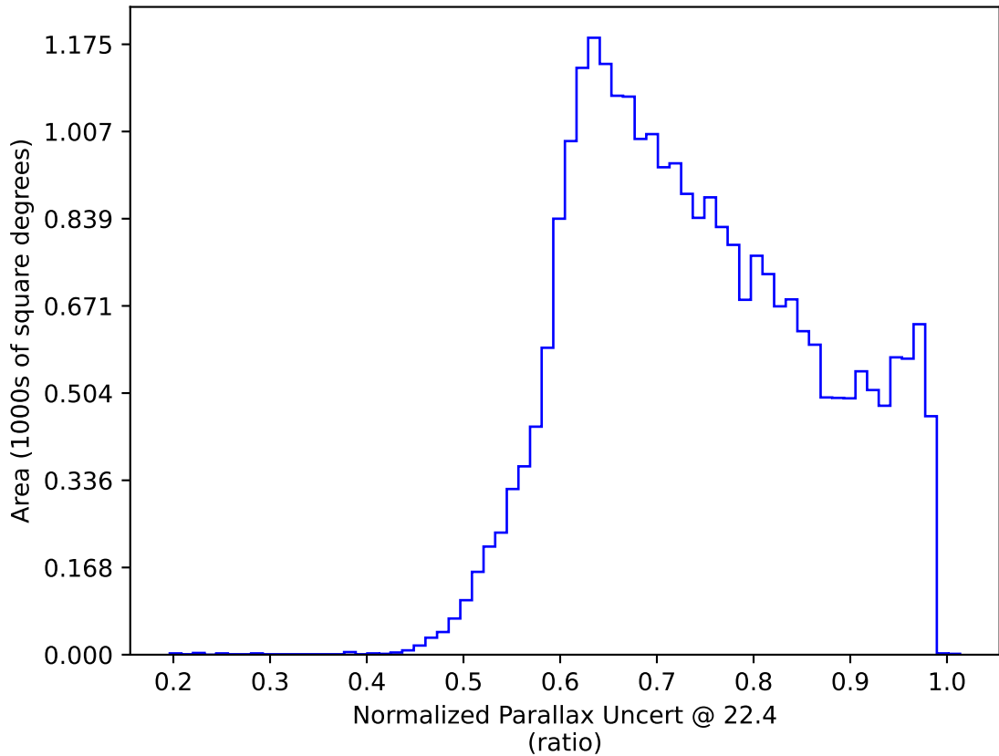
too_combined_s1.0_v3.4_10yrs : Normalized Parallax Uncert @ 22.4
