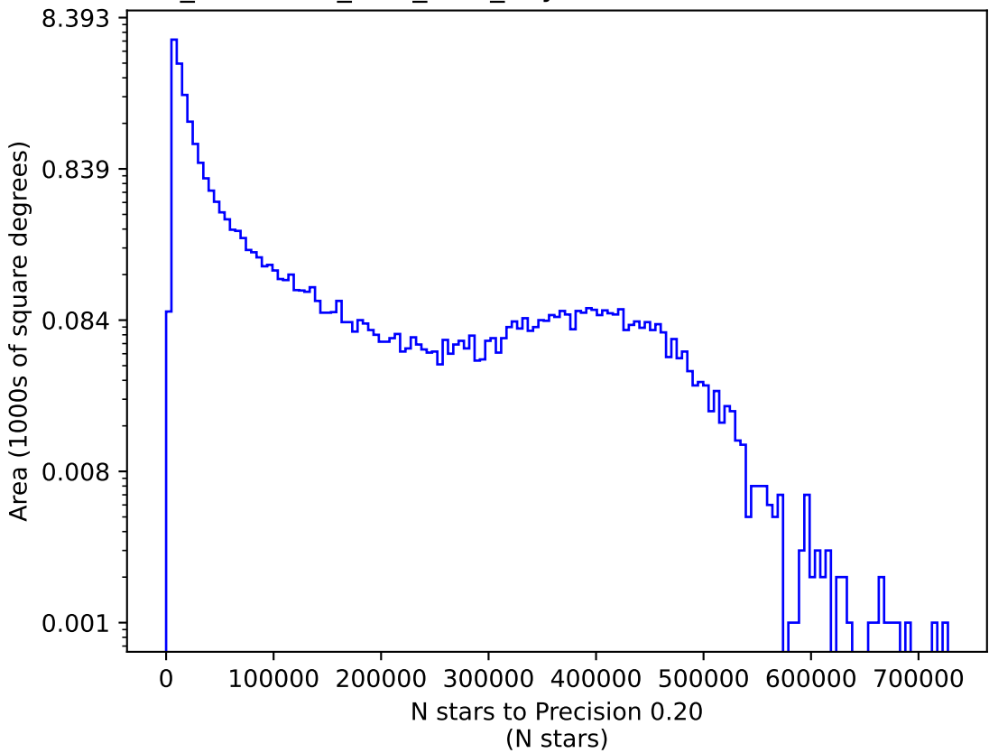
too_combined_s1.0_v3.4_10yrs z: N stars to Precision 0.20
