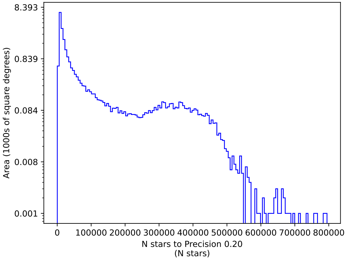
too_combined_s1.0_v3.4_10yrs y: N stars to Precision 0.20
