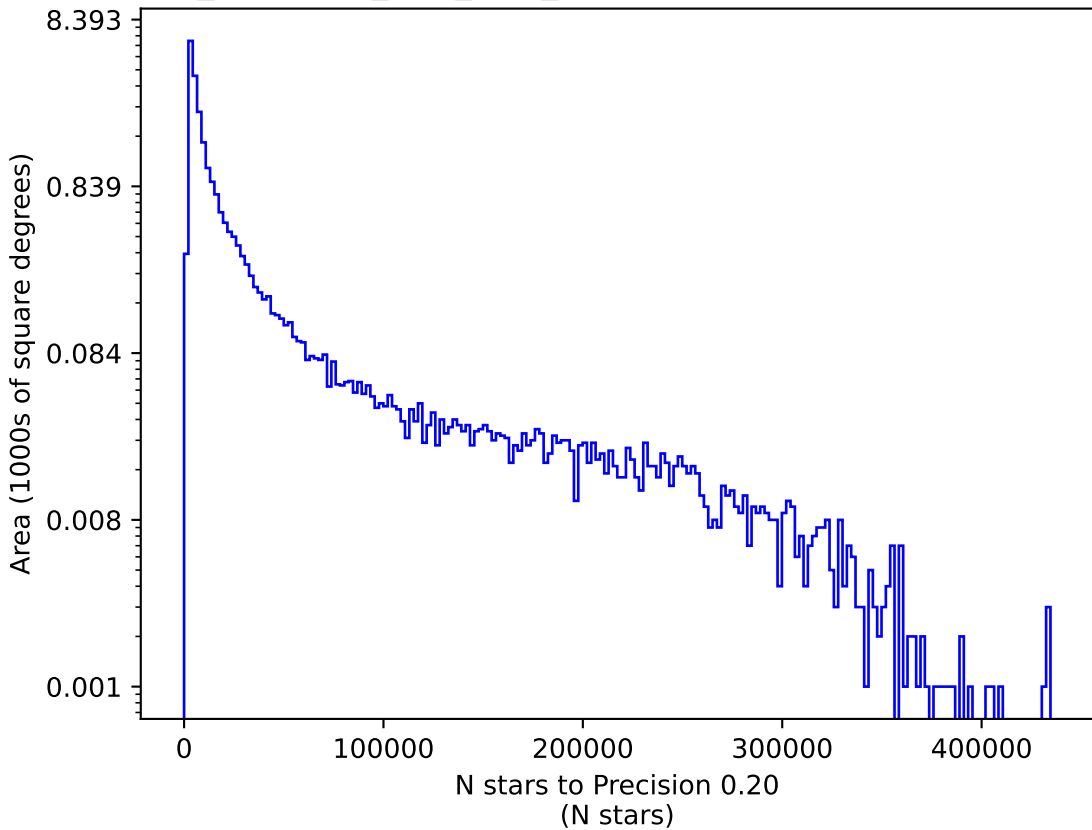
too_combined_s1.0_v3.4_10yrs u: N stars to Precision 0.20
