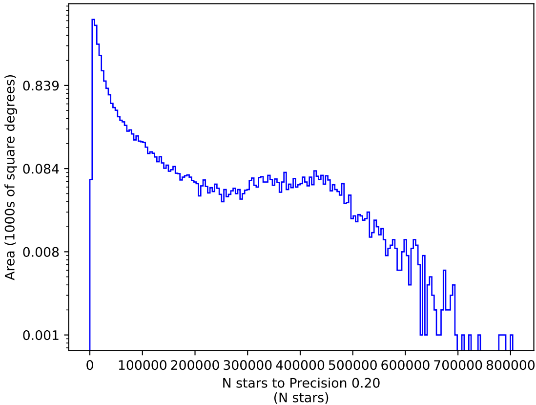
too_combined_s1.0_v3.4_10yrs r: N stars to Precision 0.20
