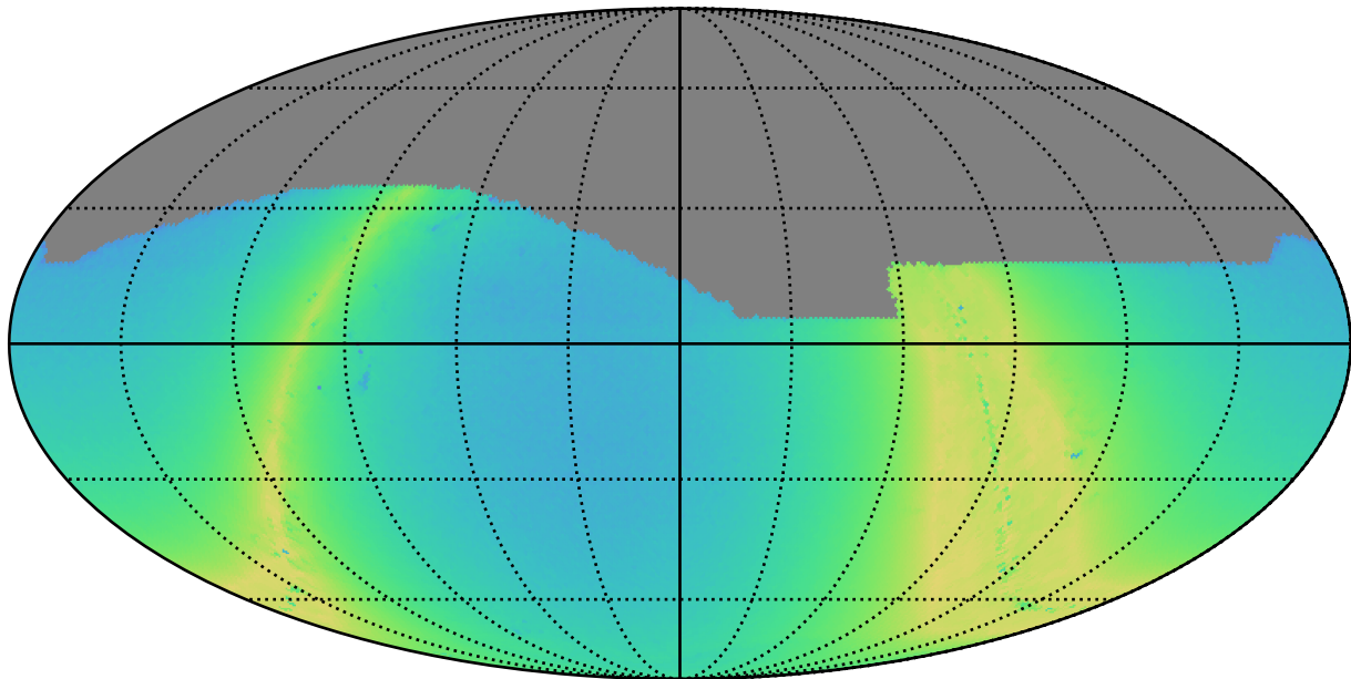
too_combined_s1.0_v3.4_10yrs i: N stars to Precision 0.20
