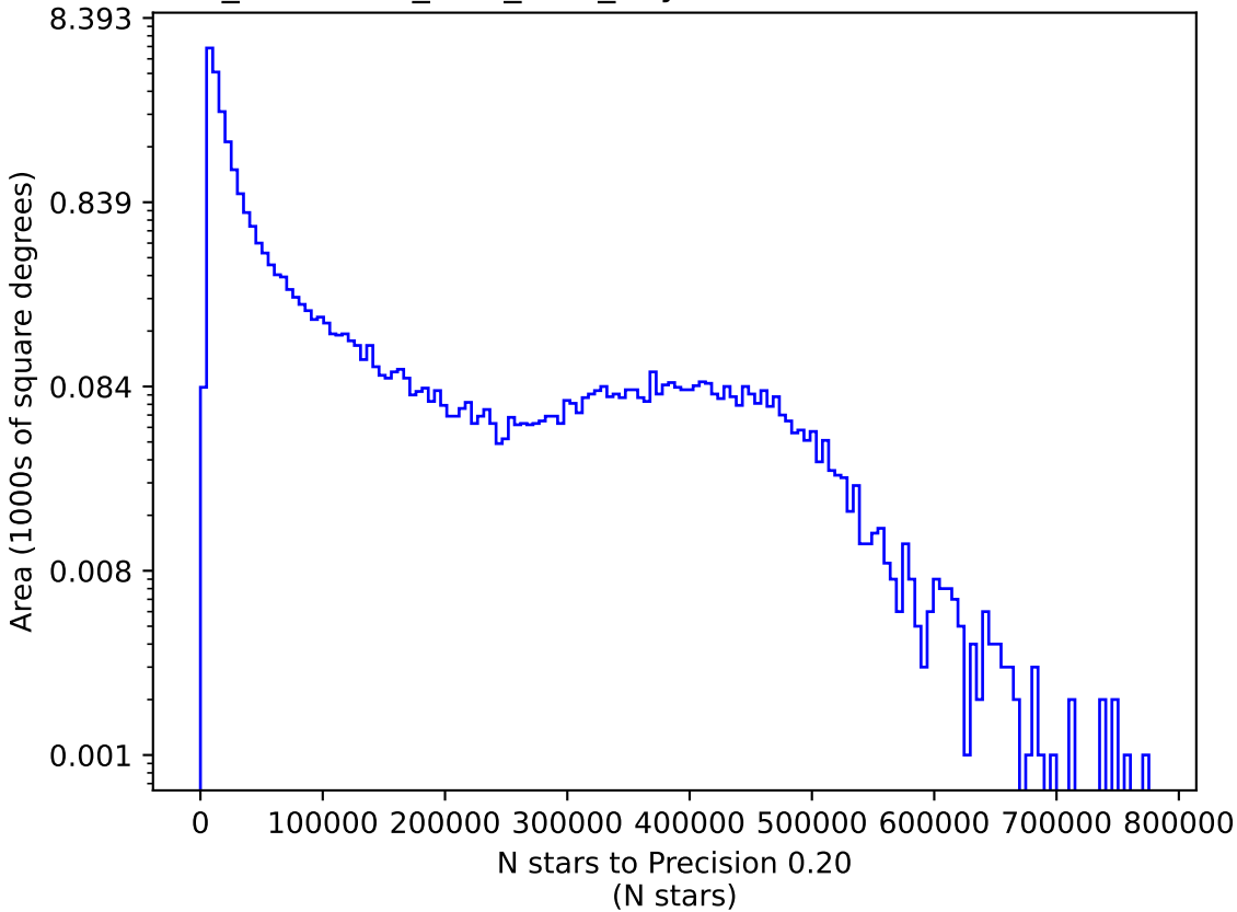
too_combined_s1.0_v3.4_10yrs i: N stars to Precision 0.20
