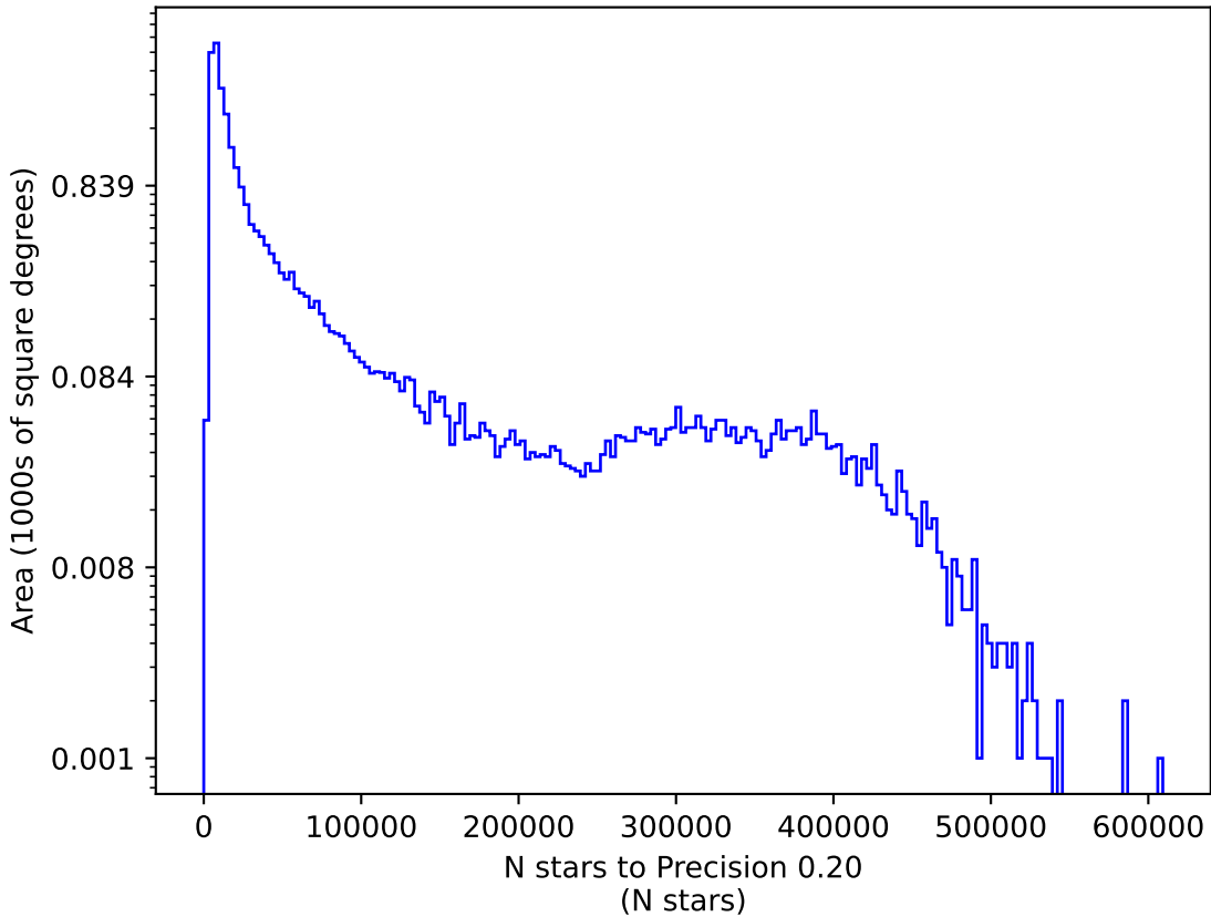
too_combined_s1.0_v3.4_10yrs g: N stars to Precision 0.20
