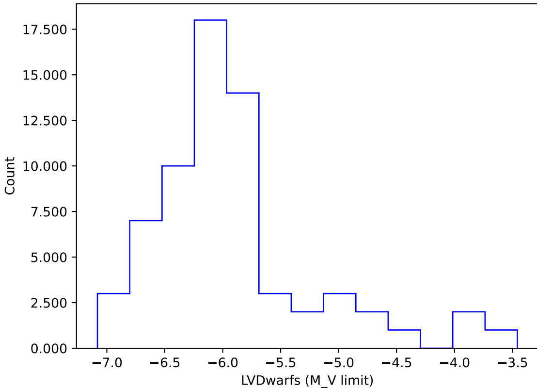
too_combined_s1.0_v3.4_10yrs gi: LVDwarfs
