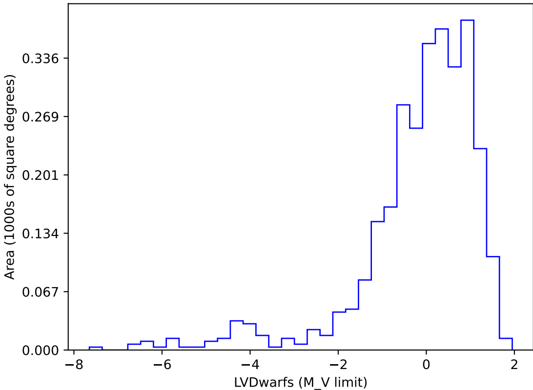
too_combined_s1.0_v3.4_10yrs gi SCP: LVDwarfs
