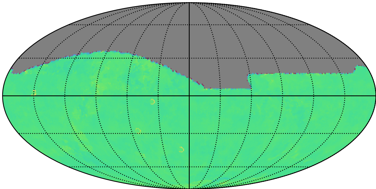
too_combined_s1.0_v3.4_10yrs z: Kuiper rotTelPos
