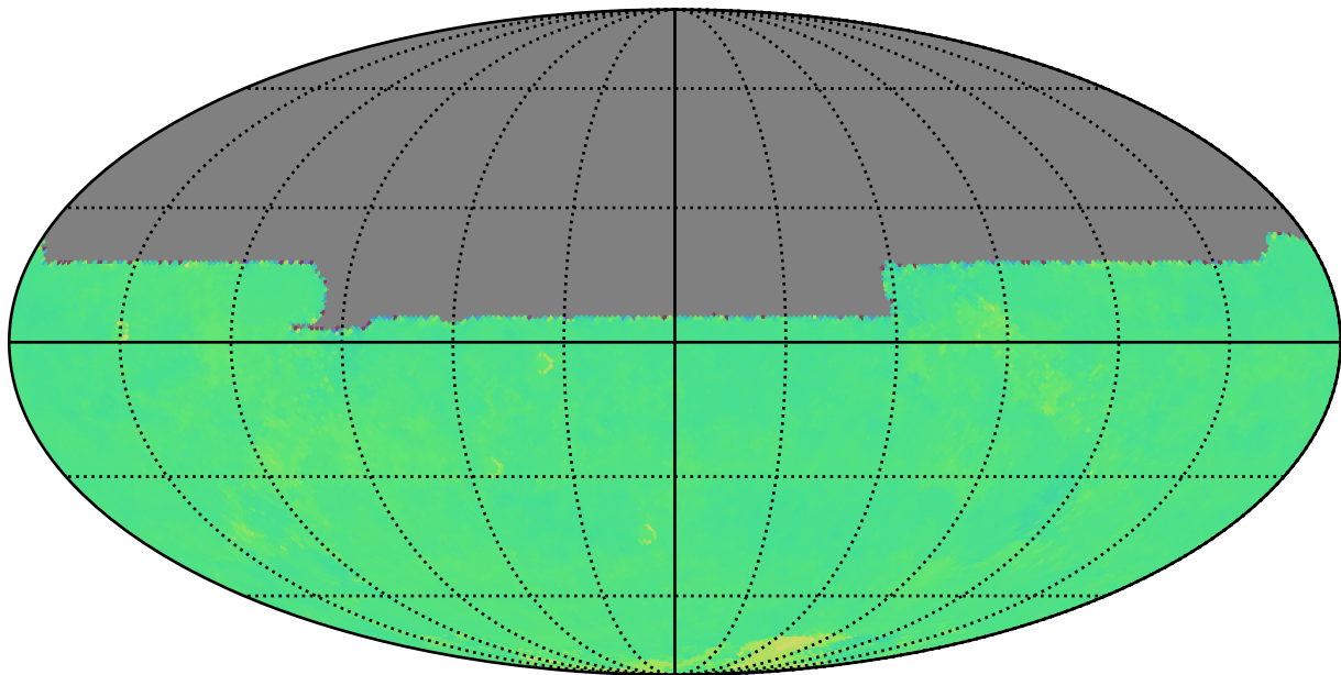
too_combined_s1.0_v3.4_10yrs y: Kuiper rotTelPos
