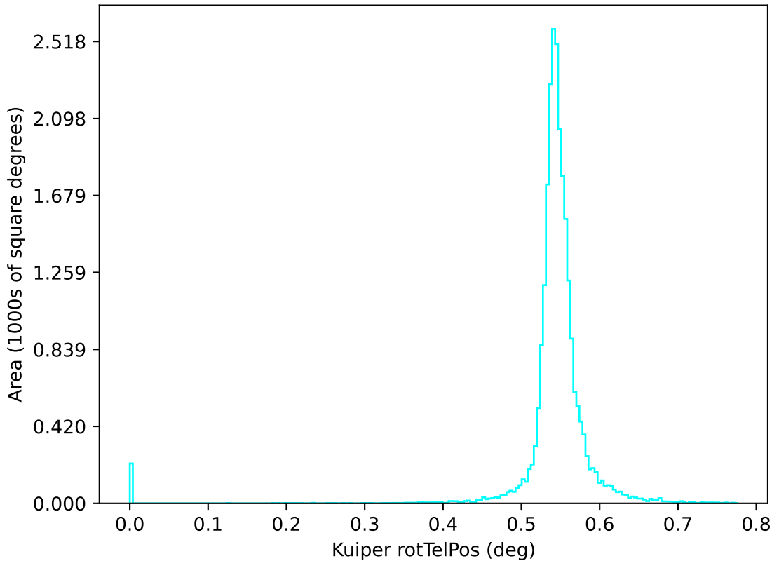
too_combined_s1.0_v3.4_10yrs u: Kuiper rotTelPos
