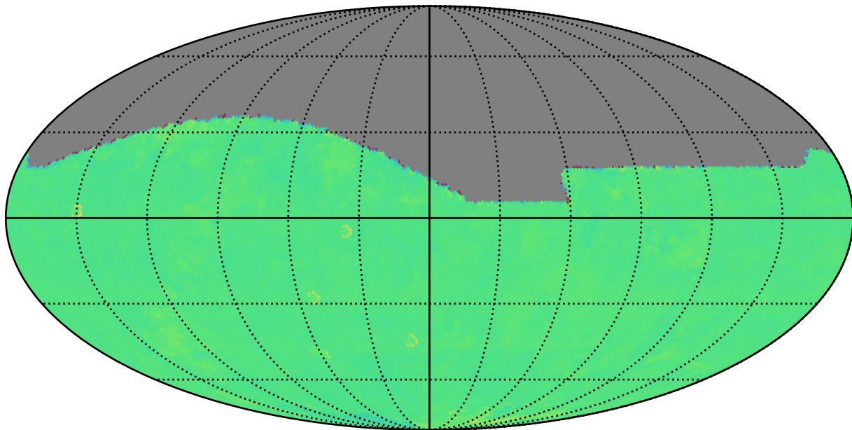
too_combined_s1.0_v3.4_10yrs r: Kuiper rotTelPos
