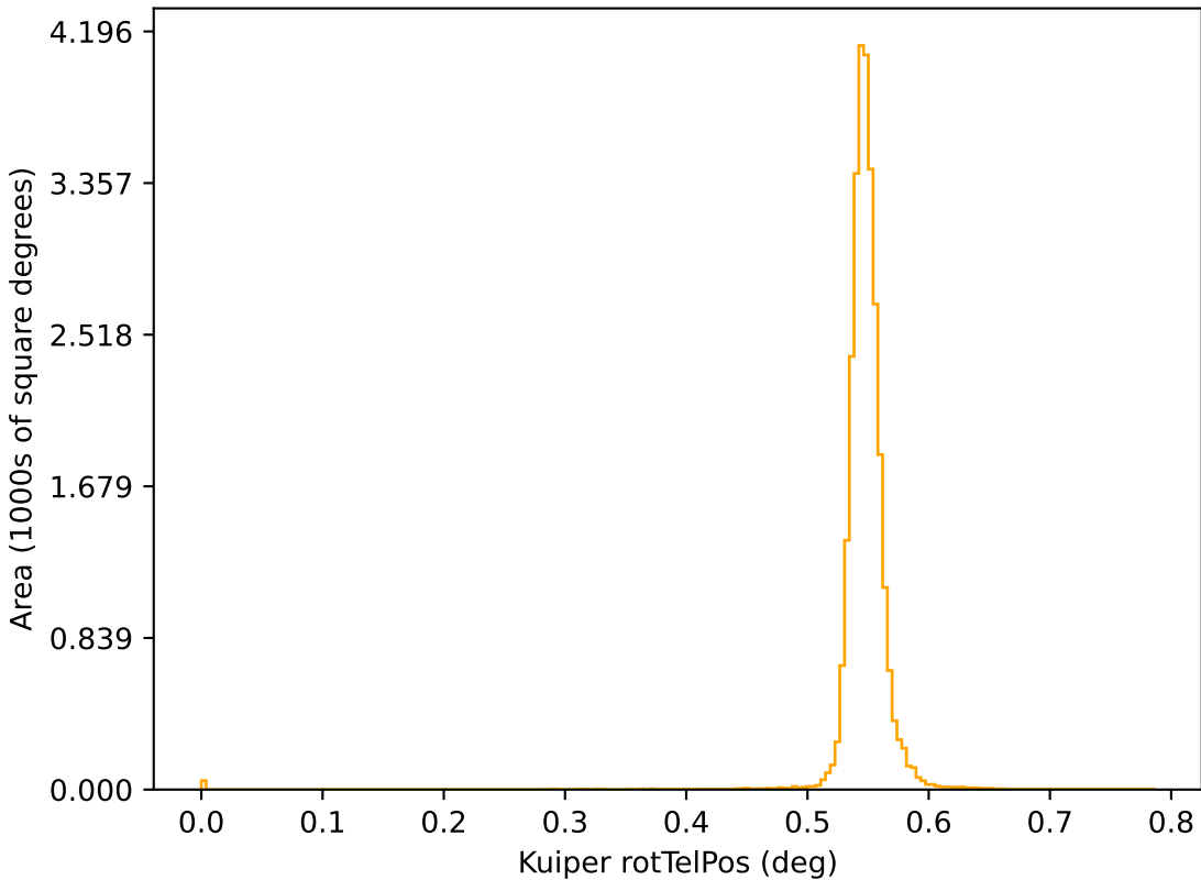
too_combined_s1.0_v3.4_10yrs r: Kuiper rotTelPos
