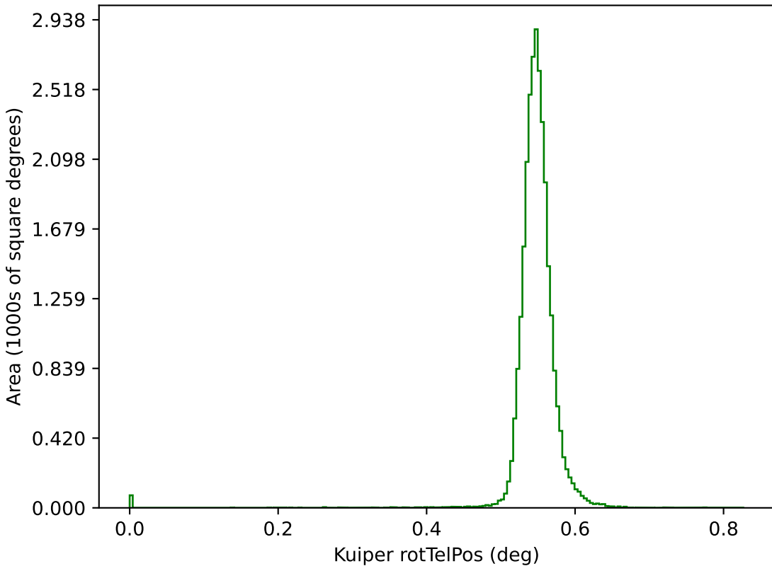
too_combined_s1.0_v3.4_10yrs g: Kuiper rotTelPos
