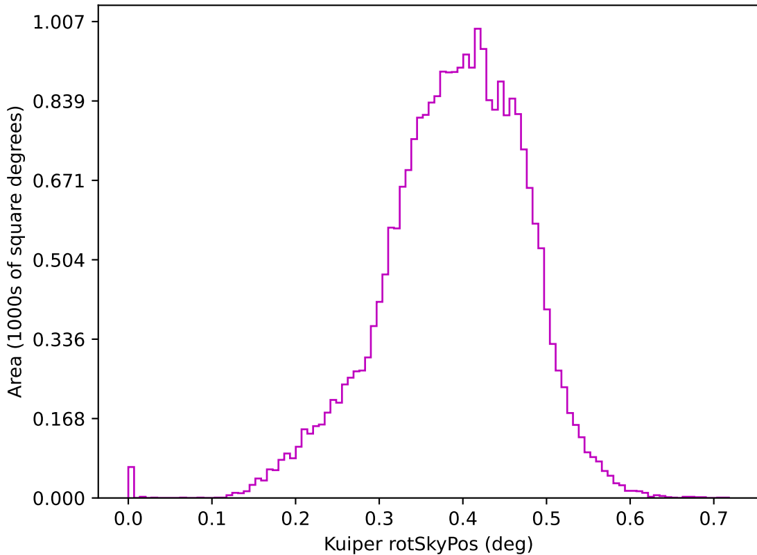
too_combined_s1.0_v3.4_10yrs z: Kuiper rotSkyPos
