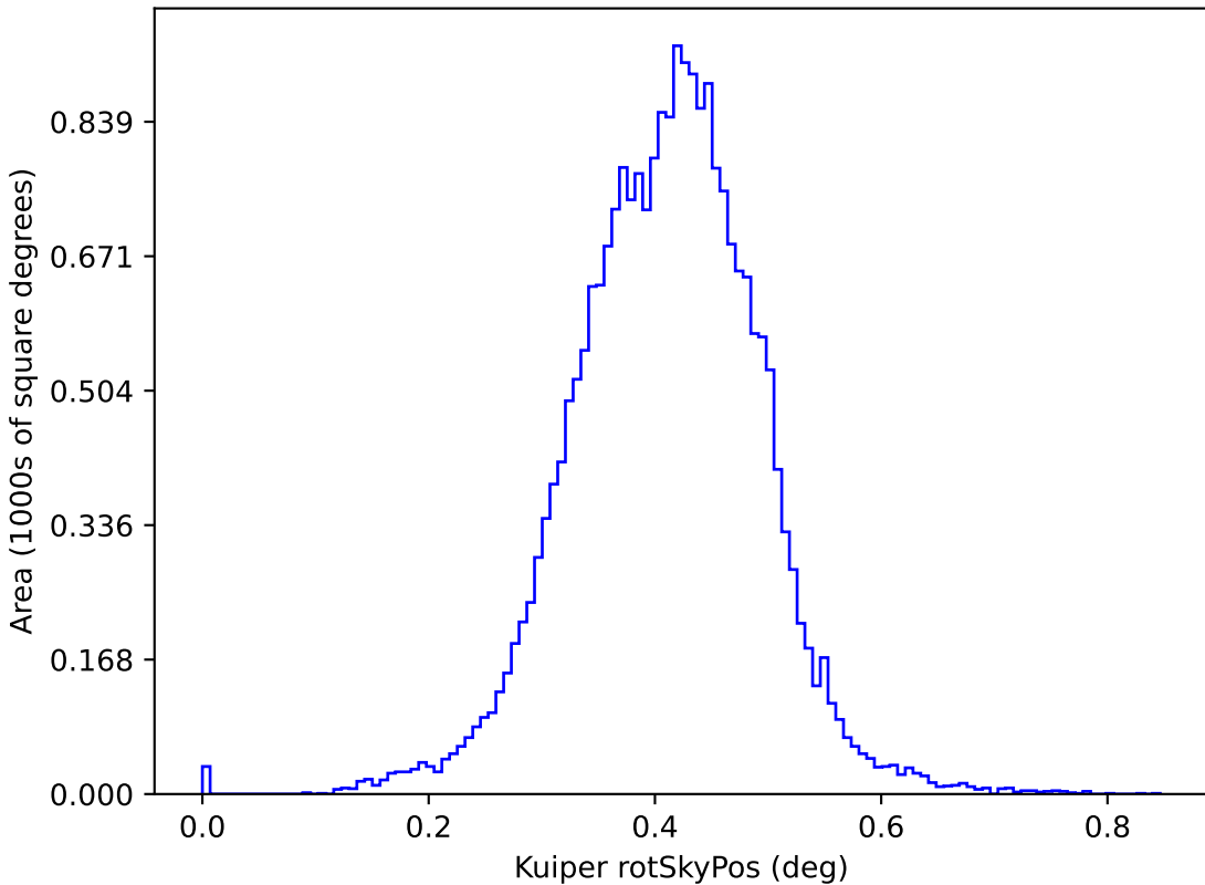
too_combined_s1.0_v3.4_10yrs y: Kuiper rotSkyPos
