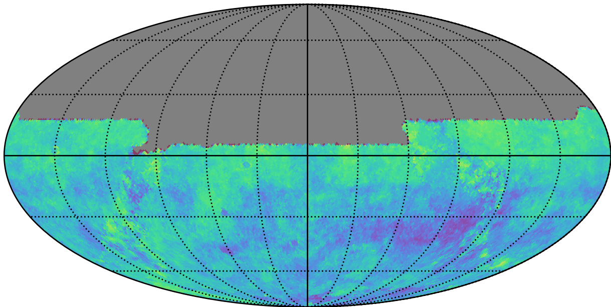
too_combined_s1.0_v3.4_10yrs u: Kuiper rotSkyPos
