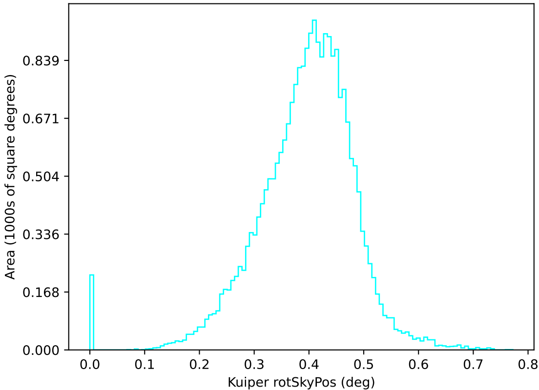
too_combined_s1.0_v3.4_10yrs u: Kuiper rotSkyPos
