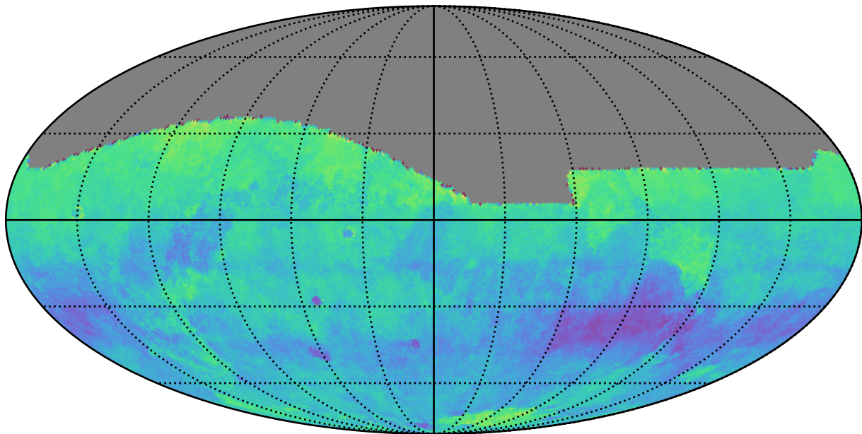
too_combined_s1.0_v3.4_10yrs r: Kuiper rotSkyPos
