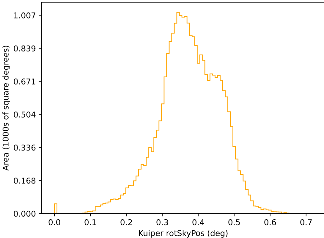
too_combined_s1.0_v3.4_10yrs r: Kuiper rotSkyPos
