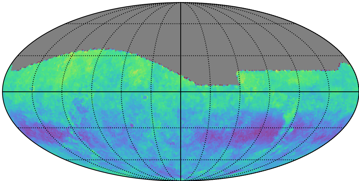
too_combined_s1.0_v3.4_10yrs g: Kuiper rotSkyPos
