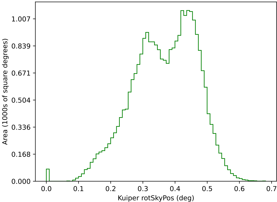
too_combined_s1.0_v3.4_10yrs g: Kuiper rotSkyPos
