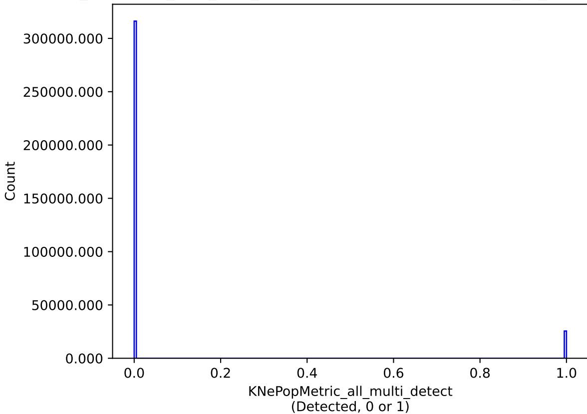
too_combined_s1.0_v3.4_10yrs all models: KNePopMetric_all_multi_detect
