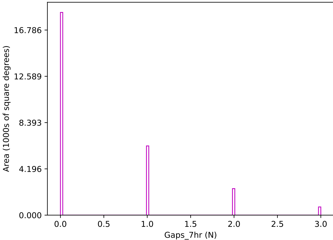
too_combined_s1.0_v3.4_10yrs z band: Gaps_7hr
