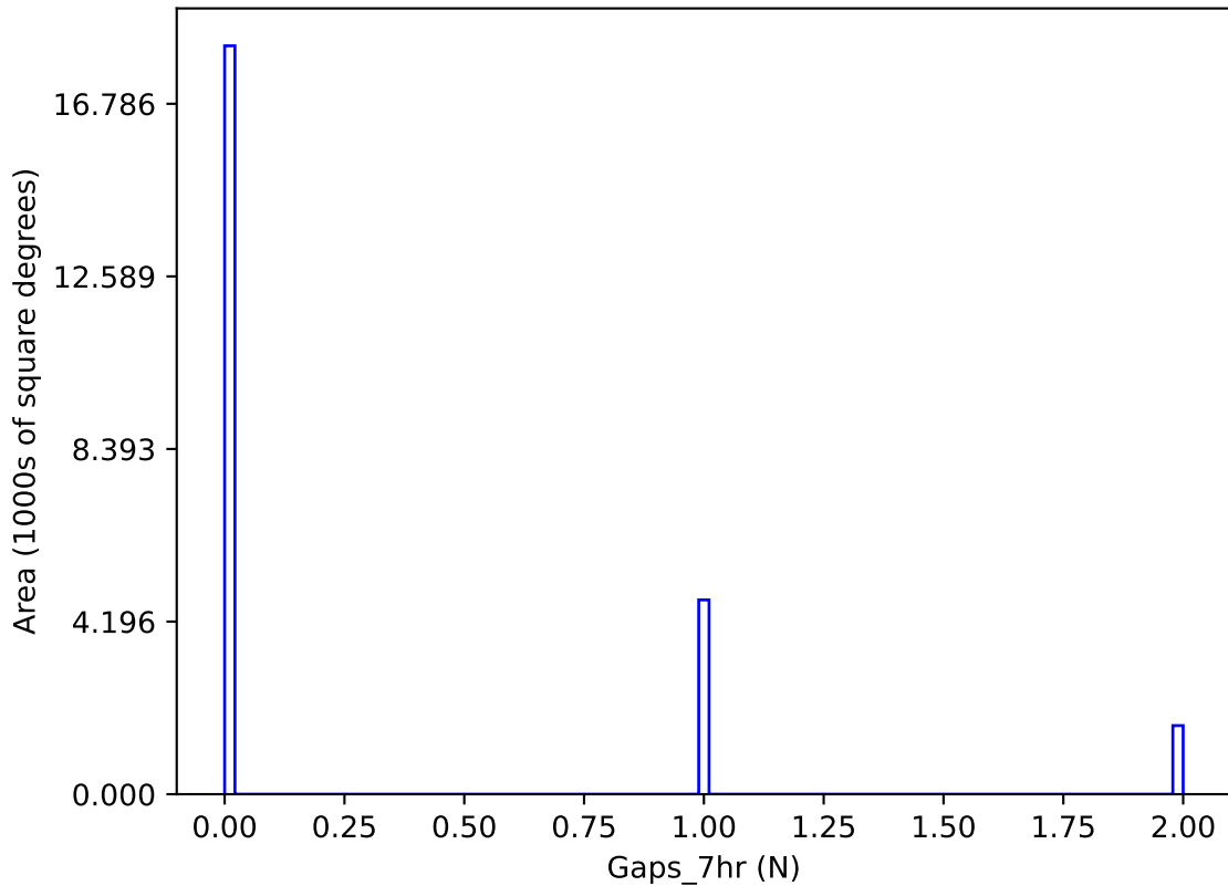
too_combined_s1.0_v3.4_10yrs y band: Gaps_7hr
