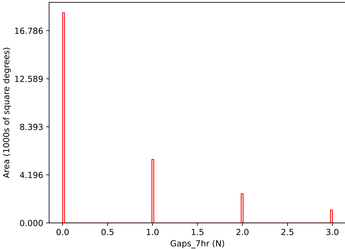
too_combined_s1.0_v3.4_10yrs i band: Gaps_7hr
