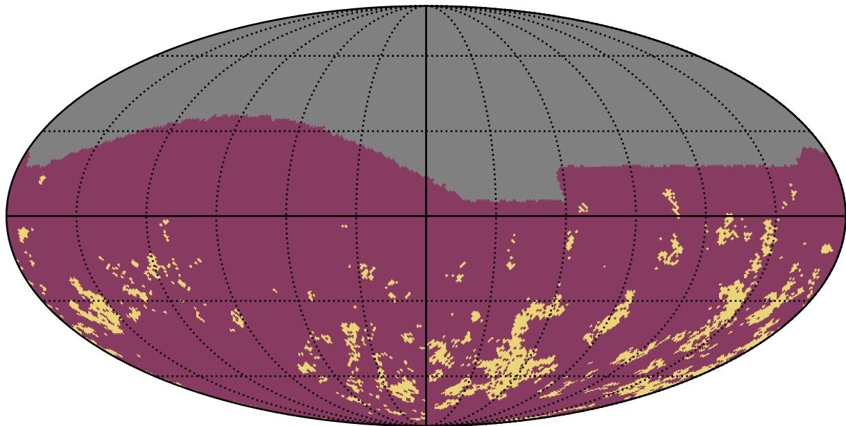
too_combined_s1.0_v3.4_10yrs g band: Gaps_7hr
