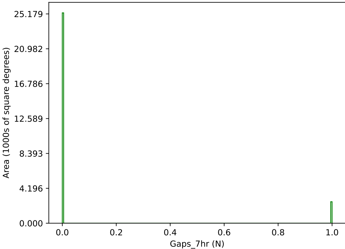
too_combined_s1.0_v3.4_10yrs g band: Gaps_7hr
