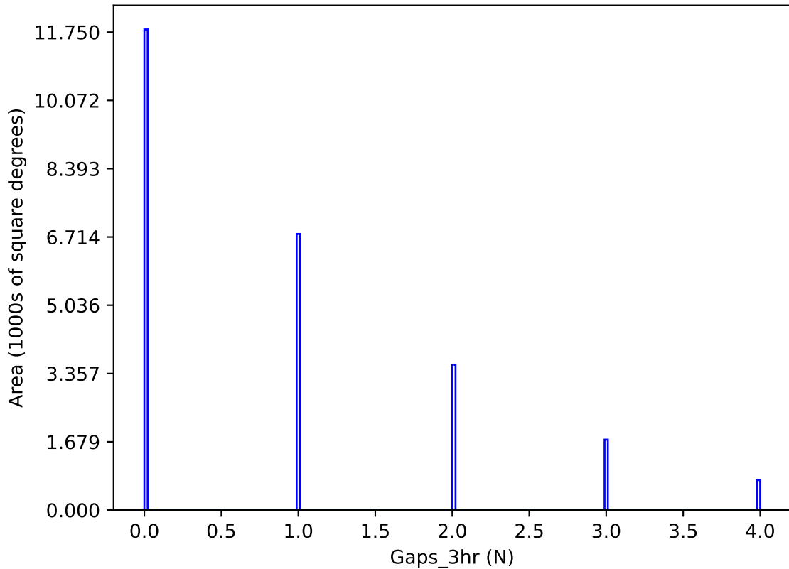
too_combined_s1.0_v3.4_10yrs y band: Gaps_3hr
