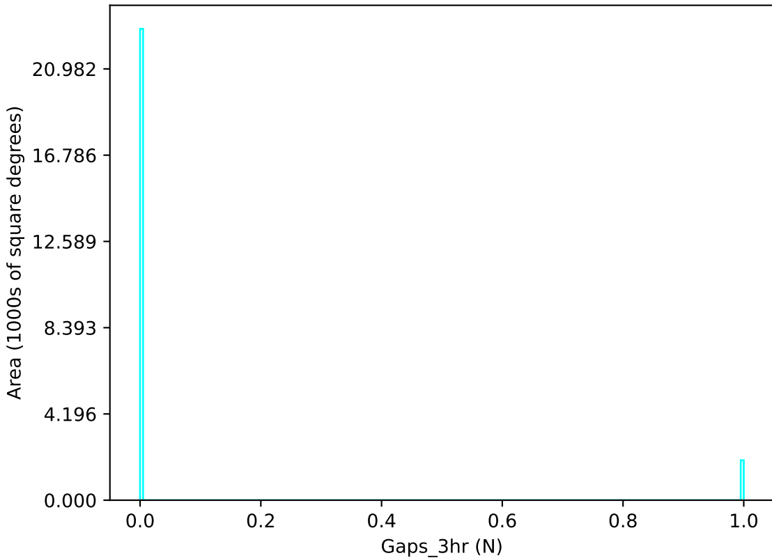
too_combined_s1.0_v3.4_10yrs u band: Gaps_3hr
