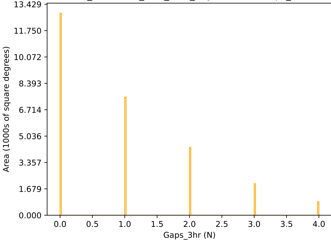
too_combined_s1.0_v3.4_10yrs r band: Gaps_3hr
