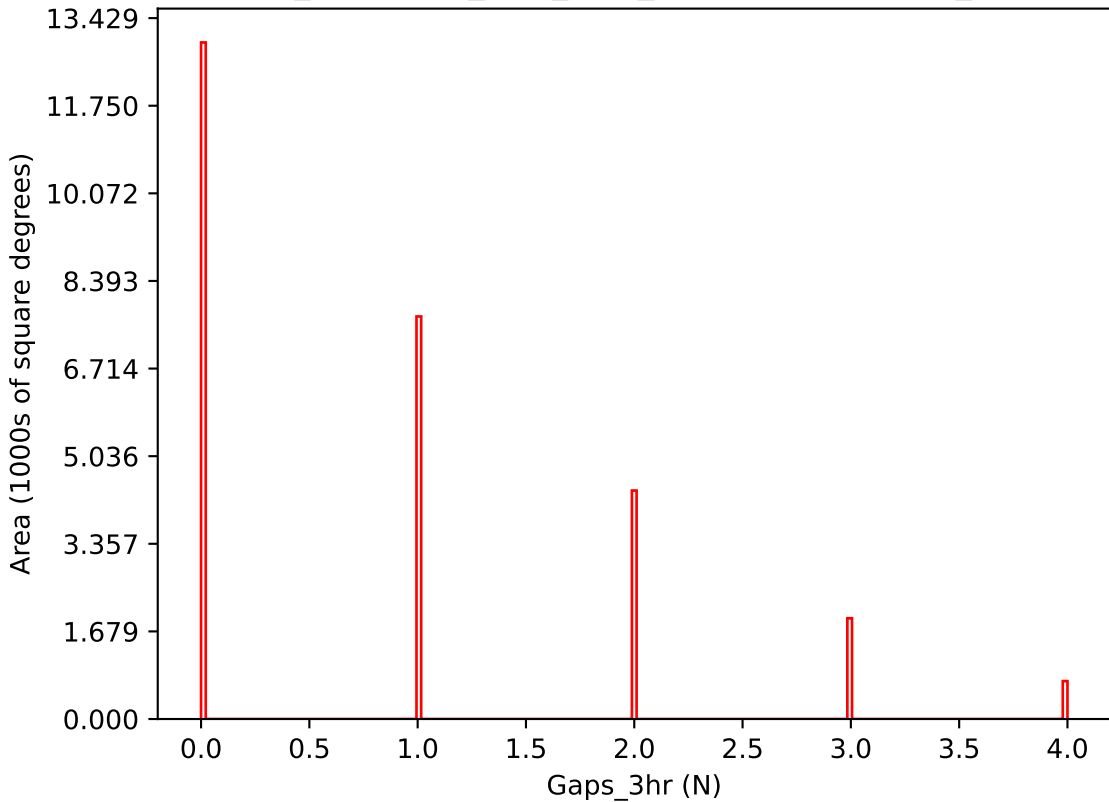
too_combined_s1.0_v3.4_10yrs i band: Gaps_3hr
