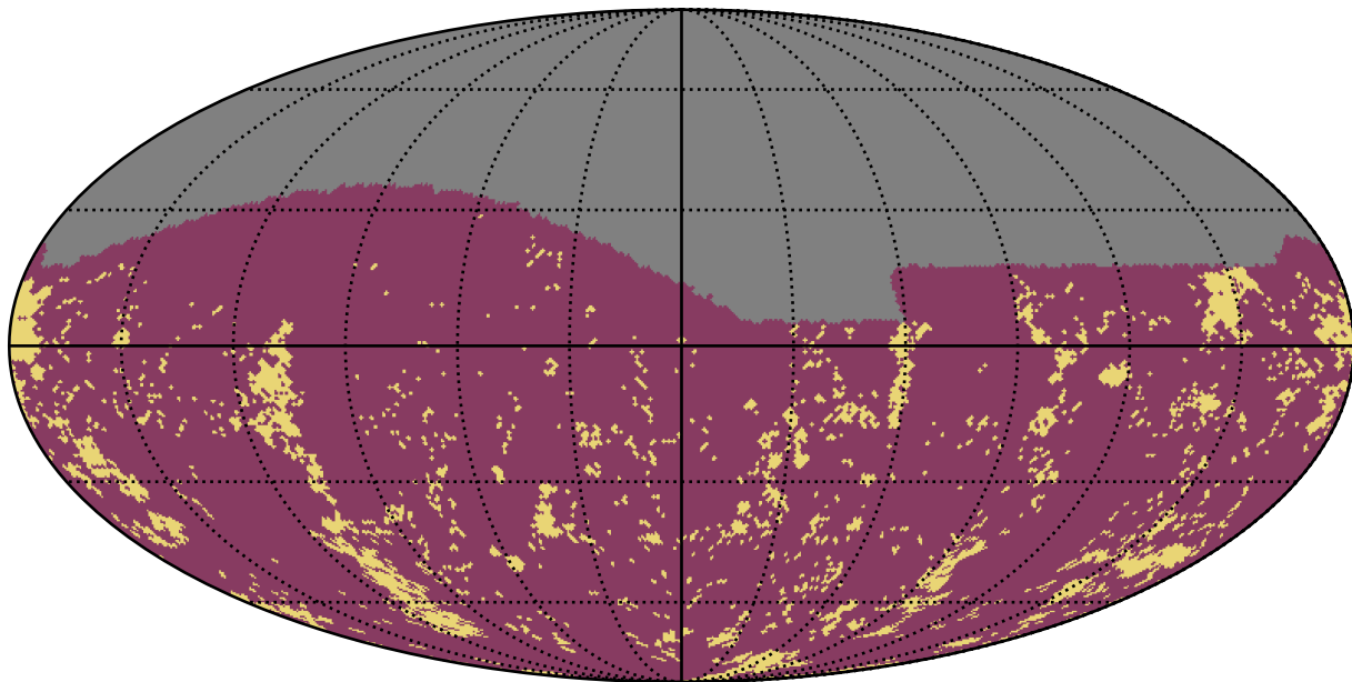
too_combined_s1.0_v3.4_10yrs g band: Gaps_3hr
