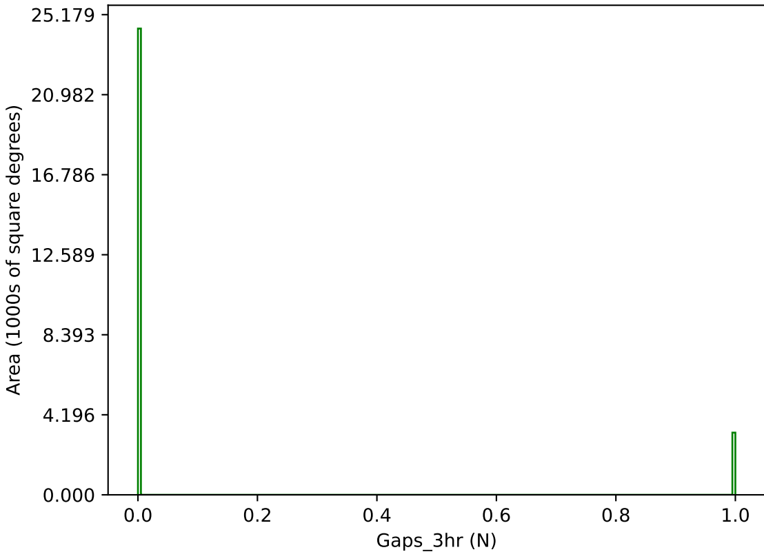
too_combined_s1.0_v3.4_10yrs g band: Gaps_3hr
