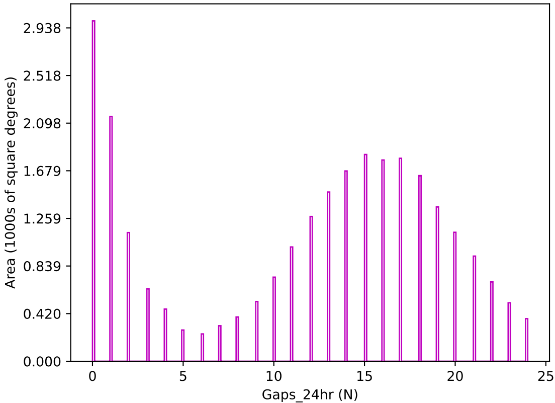
too_combined_s1.0_v3.4_10yrs z band: Gaps_24hr
