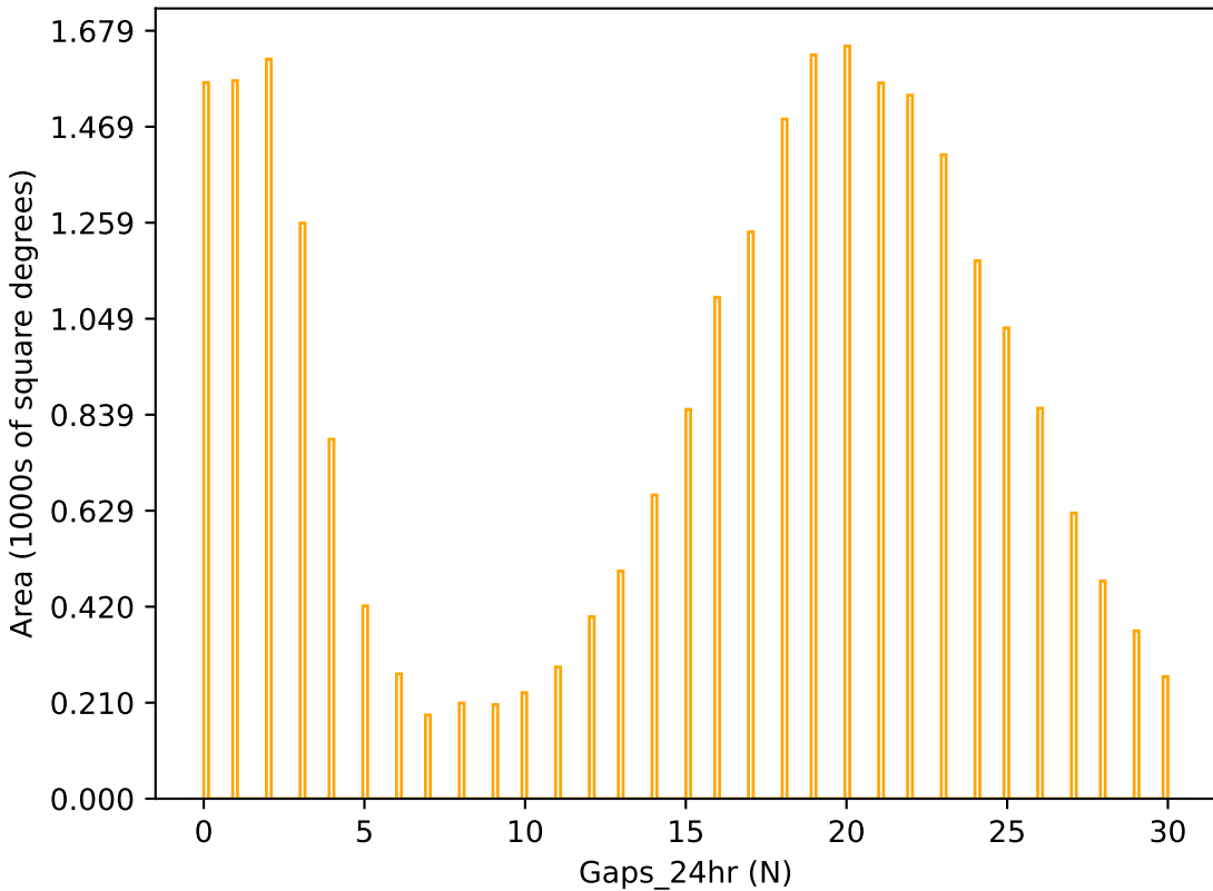
too_combined_s1.0_v3.4_10yrs r band: Gaps_24hr
