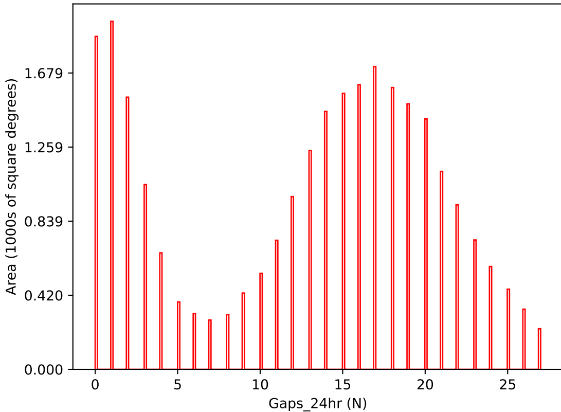
too_combined_s1.0_v3.4_10yrs i band: Gaps_24hr
